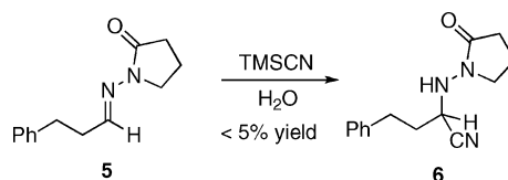
Scheme 1. Reactivity of N -acylhydrazone 5 .
