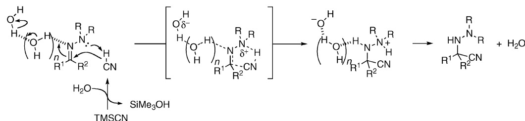
Scheme 2. Activation of cyanide for the addition to hydrazones.
