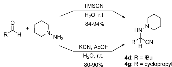
Scheme 3. One-pot, direct synthesis of hydrazino nitriles 4 from aldehydes.
