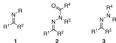
Figure 1. Imines 1 , N -acylhydrazones 2 and N,N -dialkylhydrazones 3 .
